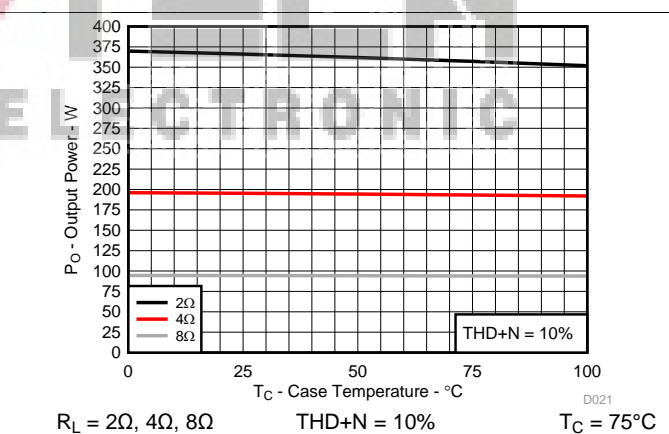
Figure 21. Output Power vs Case Temperature
