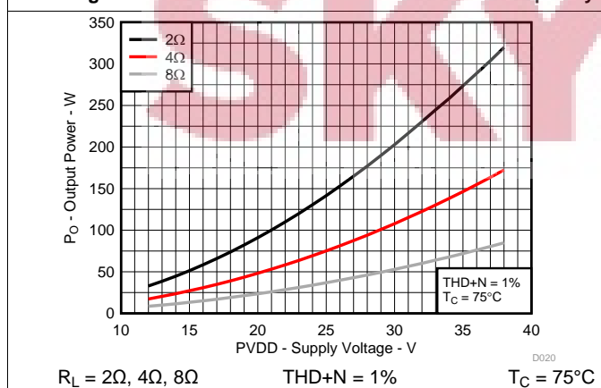
Figure 20. Output Power vs Supply Voltage
