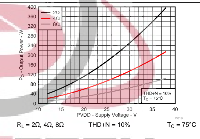
Figure 19. Output Power vs Supply Voltage
